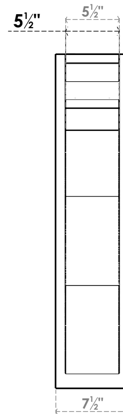
FRONT PROFILE
