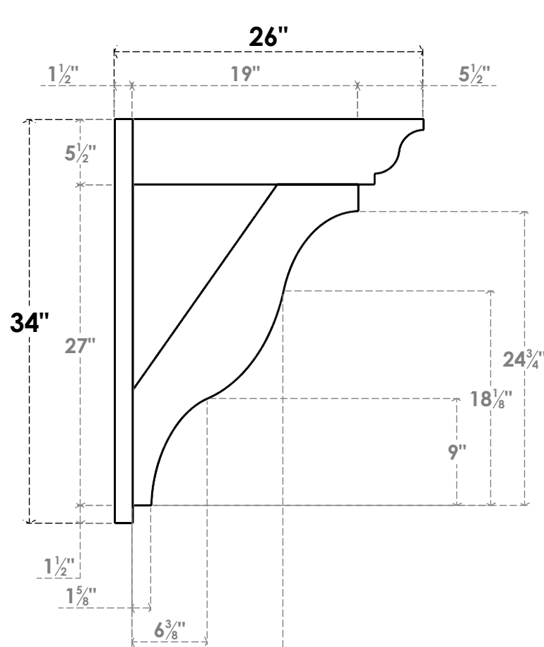
SIDE PROFILE
